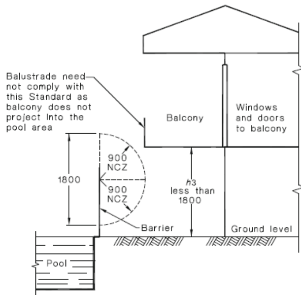
(b) Balcony adjacent pool area
