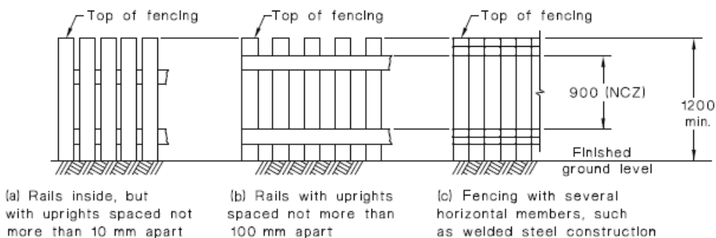
FIGURE 2.3(B) SPACING OF ACCESSIBLE HORIZONTAL MEMBERS, OR PROJECTIONS INDENTATIONS
