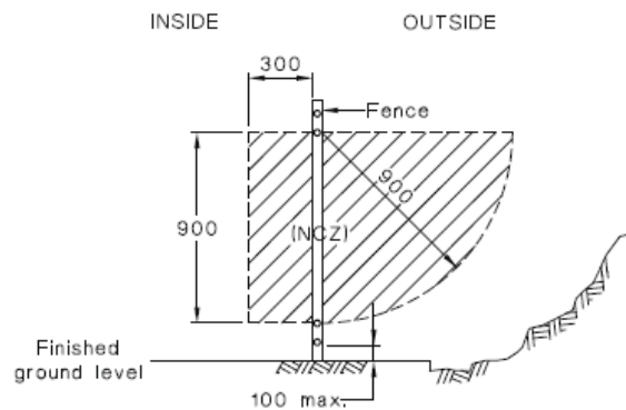
FIGURE 2.5 FENCING WITH HORIZONTAL MEMBER PROJECTIONS OR INDENTATIONS THAT MAY ACT AS A HOLD FOR CLIMBING
