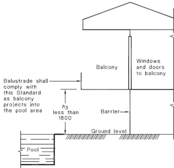
(a) Balcony projecting into pool area
