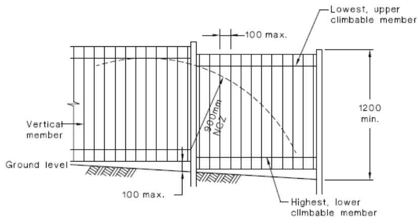
(c) Slightly sloping ground
