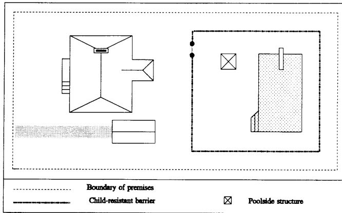
Figure 4: Boundary fencing used together with a fence to isolate the pool from the dwelling. (Boundary fences used as part of the pool barrier must comply with AS 1926.1-2007)
