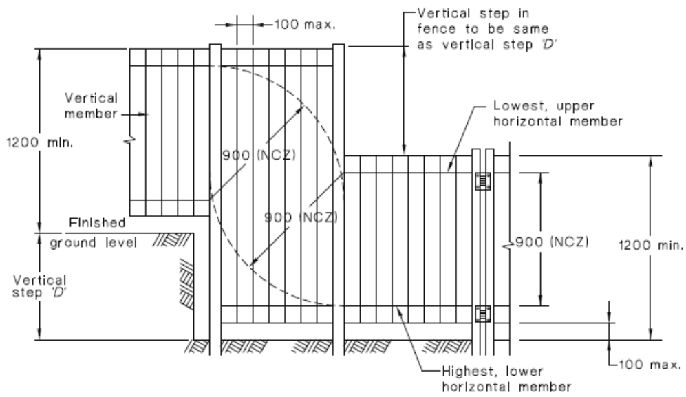
(b) Stepped ground
