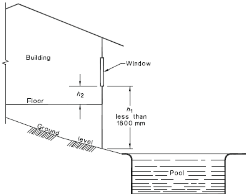
FIGURE 2.8 HEIGHT LIMITATIONS ON CHILD-RESISTANT WINDOWS
